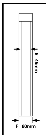
Side Elevation
